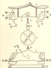
Exploded View Showing Each Part in Proper Position
